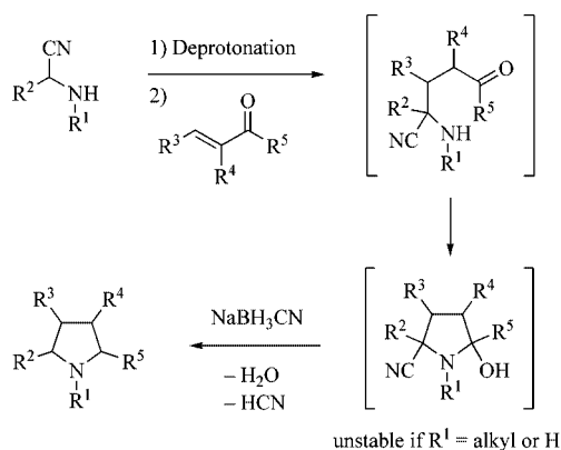
Scheme 1. Synthesis of pyrrolidines from \alpha -amino nitriles.
